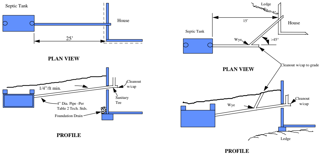
Figure 1 - Building Sewers
