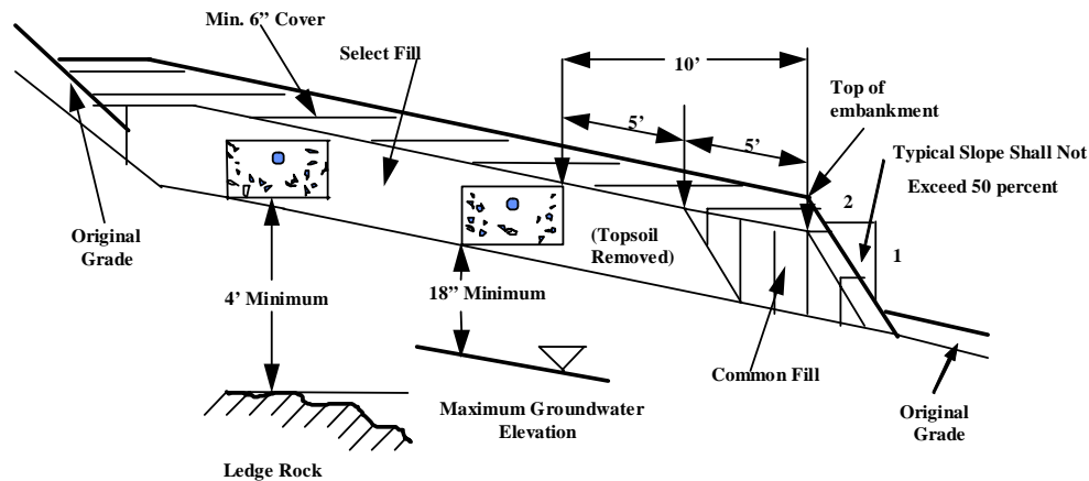
Figure 13 - Minimum Separating Distances Above Ledge Rock and Maximum Groundwater
