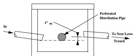
Reversed Distribution Box
