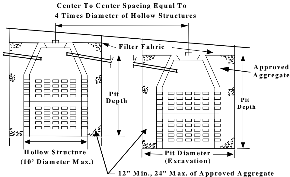
Figure 15 - Leaching Pits
