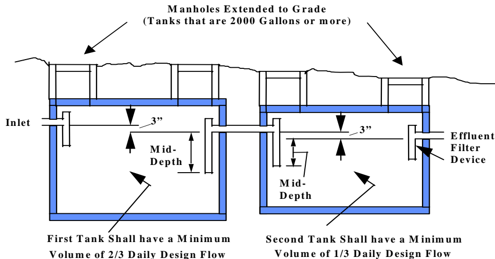
Figure 5 - Septic Tanks in Series
