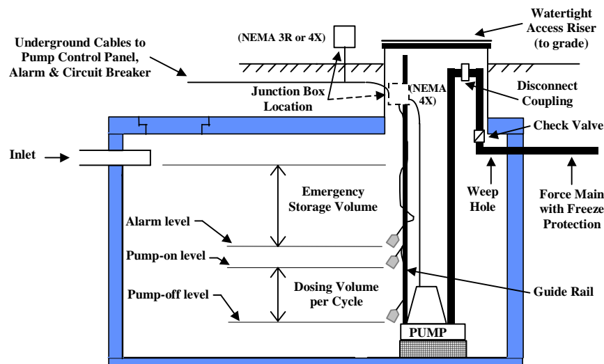
Figure 11 - Pump Chamber
