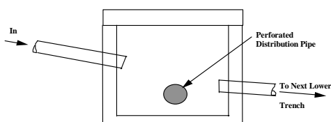
High - Level Overflow Dist. Box
