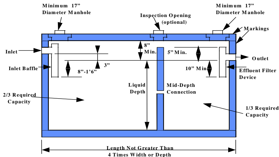
Figure 4 – Typical Septic Tank
