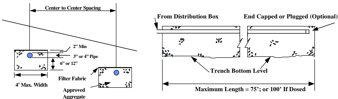
Figure 14 - Leaching Trenches
