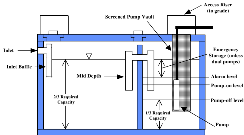
Figure 12 - Combination Septic Tank/Pump System with Tee Baffle Connection
