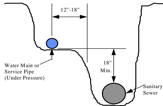
Figure 2 - Water Pipe Trenches
