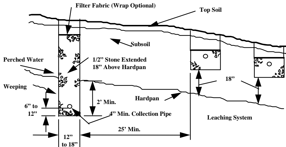
Figure 17 - Typical Curtain Drain Construction
