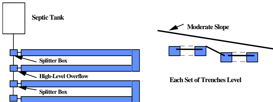
Figure 10 - Alternative Distribution Systems
