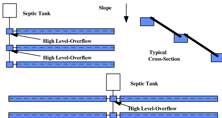
Figure 9 - Serial Distribution Boxes and Systems
