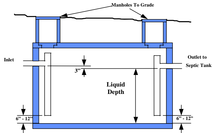
Figure 7 - Grease Interceptor Tank
