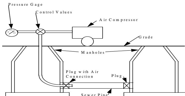
Figure 3 - Typical Air Test Equipment Layout
