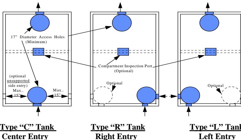
Figure 6 – Standard Septic Tank Configurations
