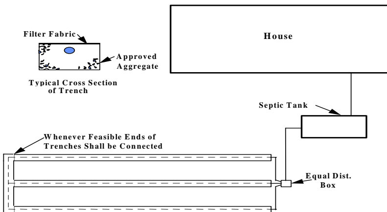
Figure 8 - Level Leaching Systems
